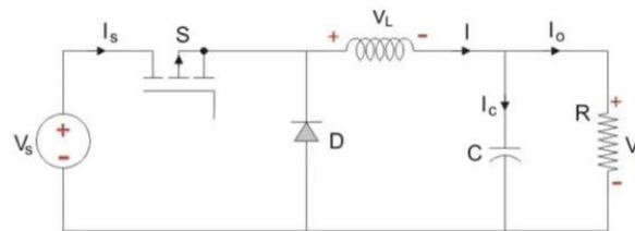
Fig 4. Buck Converter
