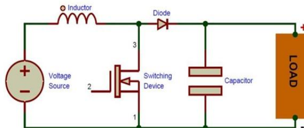
Fig 5. Boost Converter
