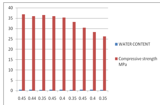
Fig. 4 Compressive strength verses water cement ratio
